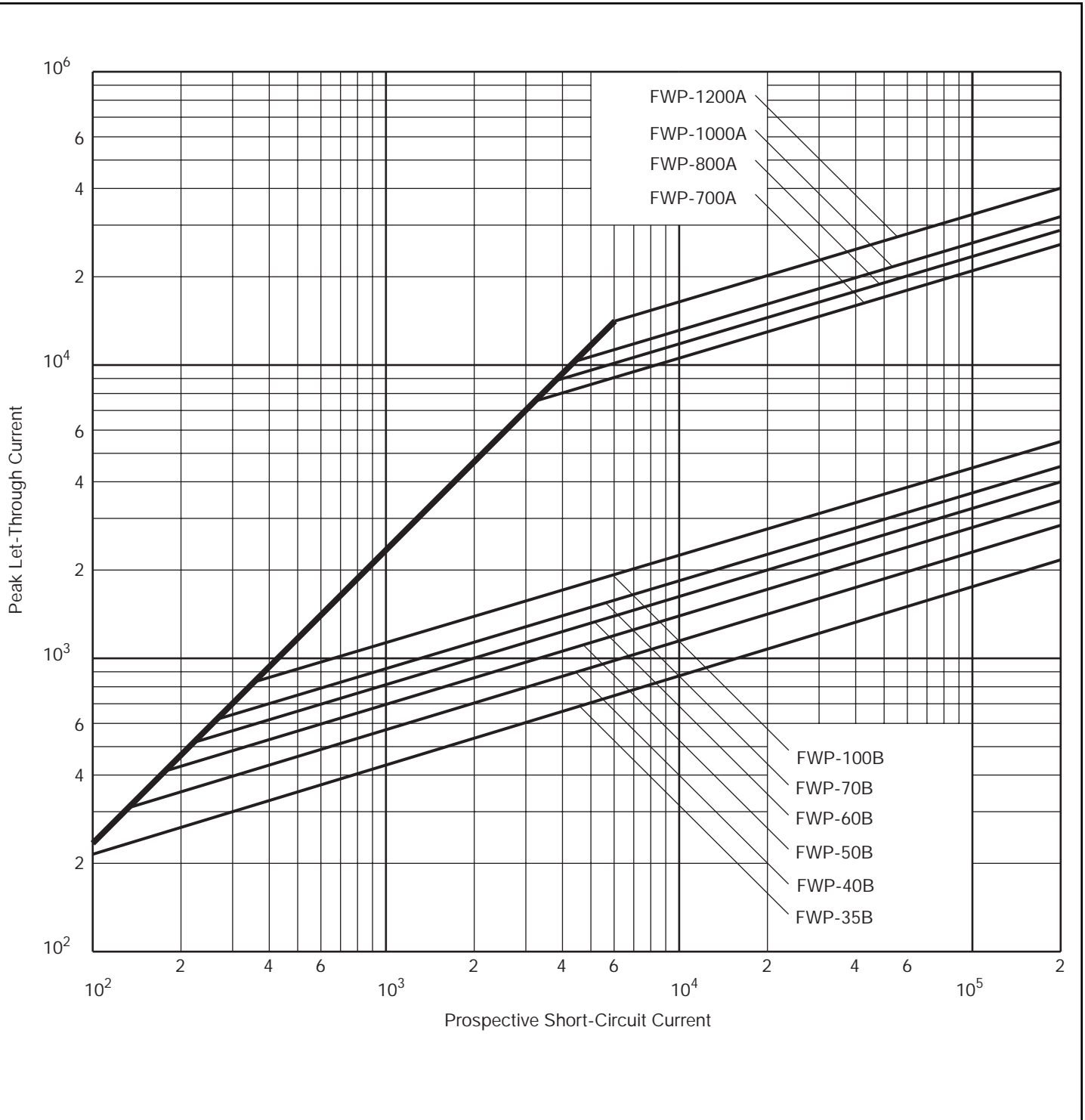
Peak Let-Through Cut-Off Current Characteristic Curves FWP 35B-100B & 700A-1200A
